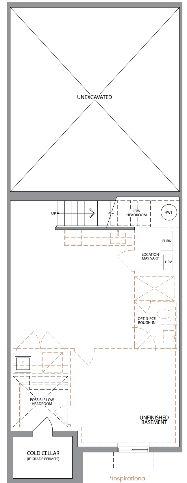
BASEMENT ELEVATION A2
